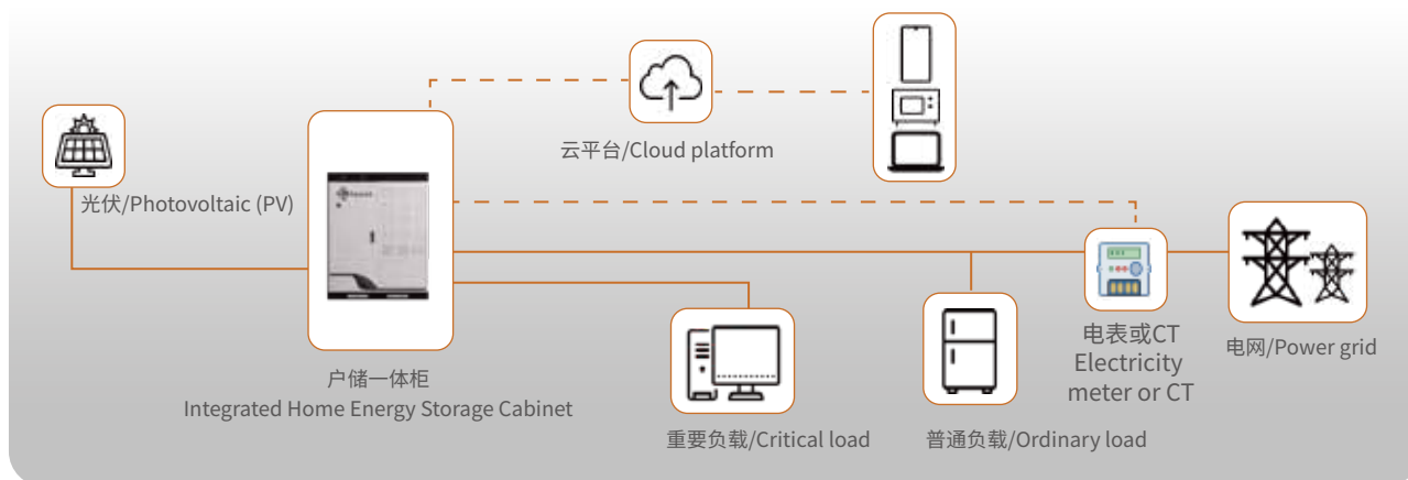
System Diagram
